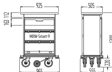
Other dimensions for MBW-Smart as on fold-out page 13.
